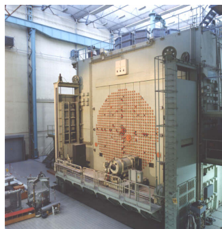
BR1 reactor
