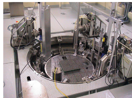
VENUS reactor
