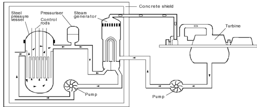
Schematic view of a PWR
